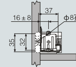
塑料后连接件 Plastic rear mounting bracket
